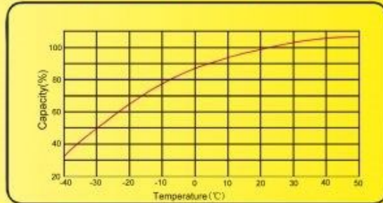
Effect of temperature on capacity
