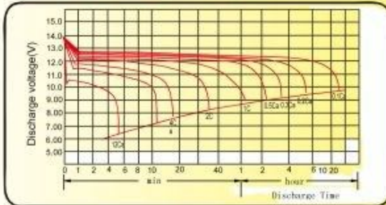
Discharge Characteristic Curve
