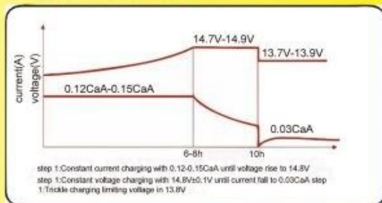
Charge Characteristic Curve
